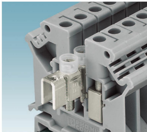
Figure 11 Fixed bridge
